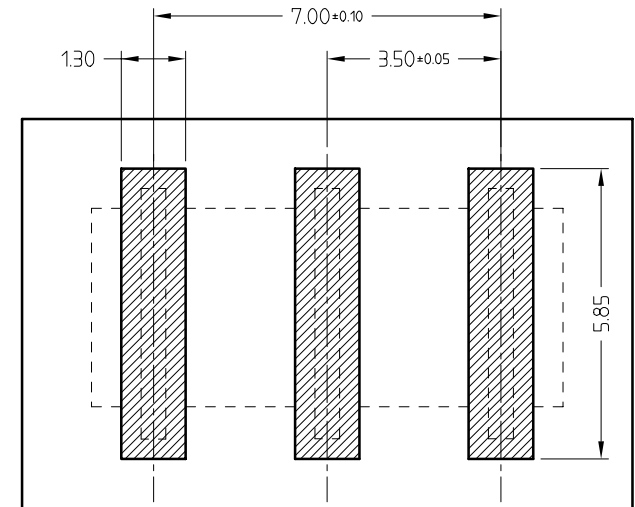
RECOMMENDED PC BOARD LAYOUT TOLERANCE: ±0.05(TOP VIEW)
