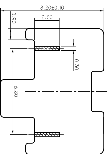
PCB LAYOUT(TOP VIEW) (TOLERANCE:±0.05)
