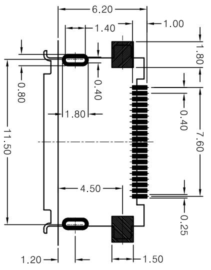
PCB LAYOUT(TOP VIEW) (TOLERANCE:±0.05)
